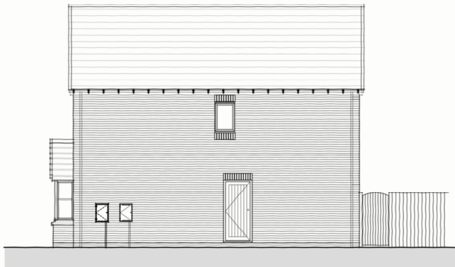
REAR ELEVATION
